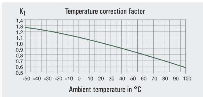
Figure 1 This curve shows the influence of the ambient temperature on the fuse's current-carrying capability.
